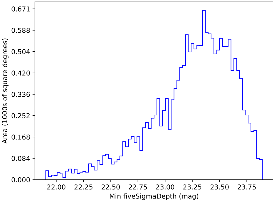
early_u_fpextra3.0_v3.4_10yrs WFD g band: Min fiveSigmaDepth
