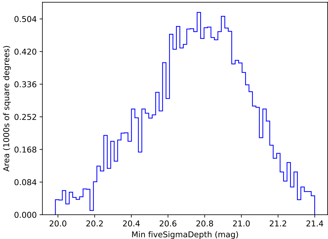
early_u_fpextra3.0_v3.4_10yrs WFD all bands: Min fiveSigmaDepth
