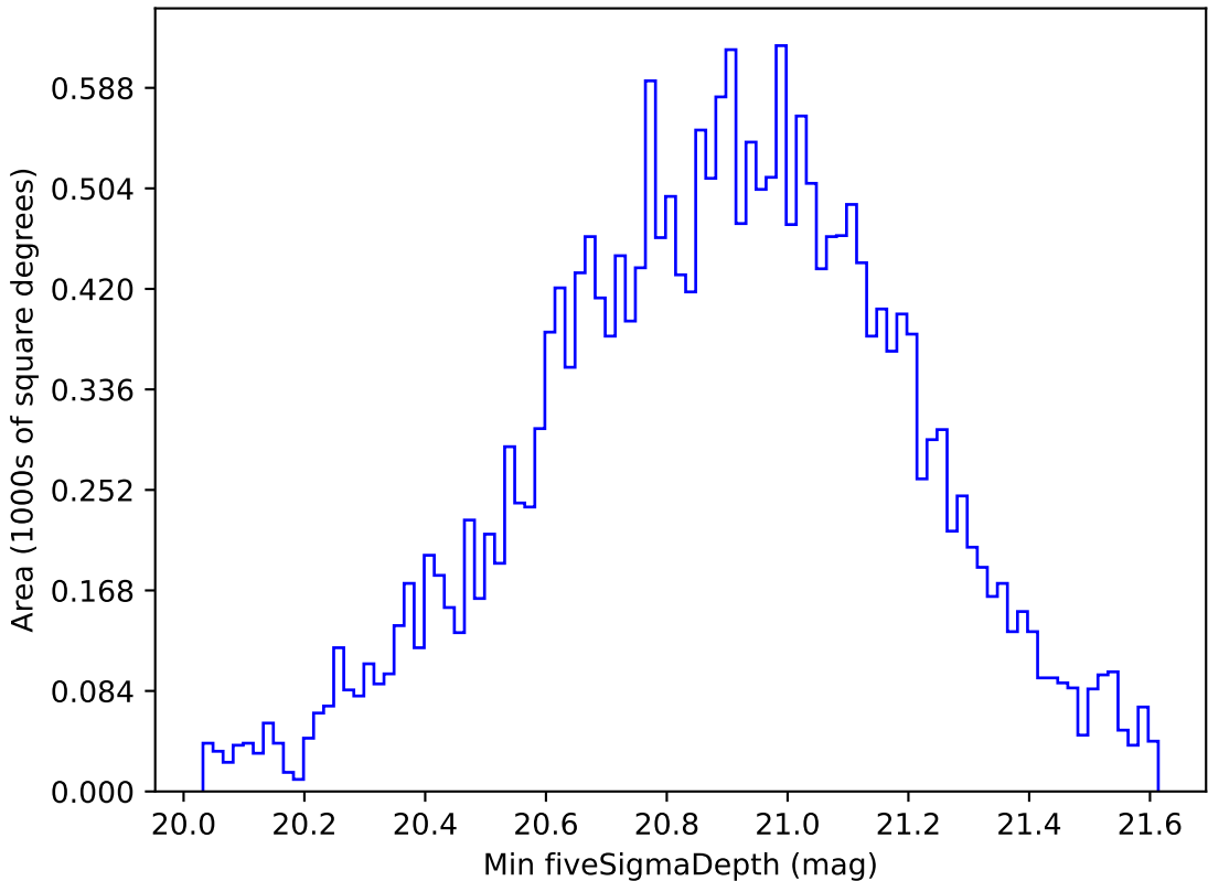
early_u_fpextra3.0_v3.4_10yrs All sky y band: Min fiveSigmaDepth
