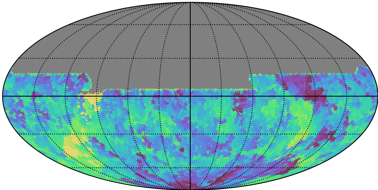
early_u_fpextra3.0_v3.4_10yrs All sky u band: Min fiveSigmaDepth
