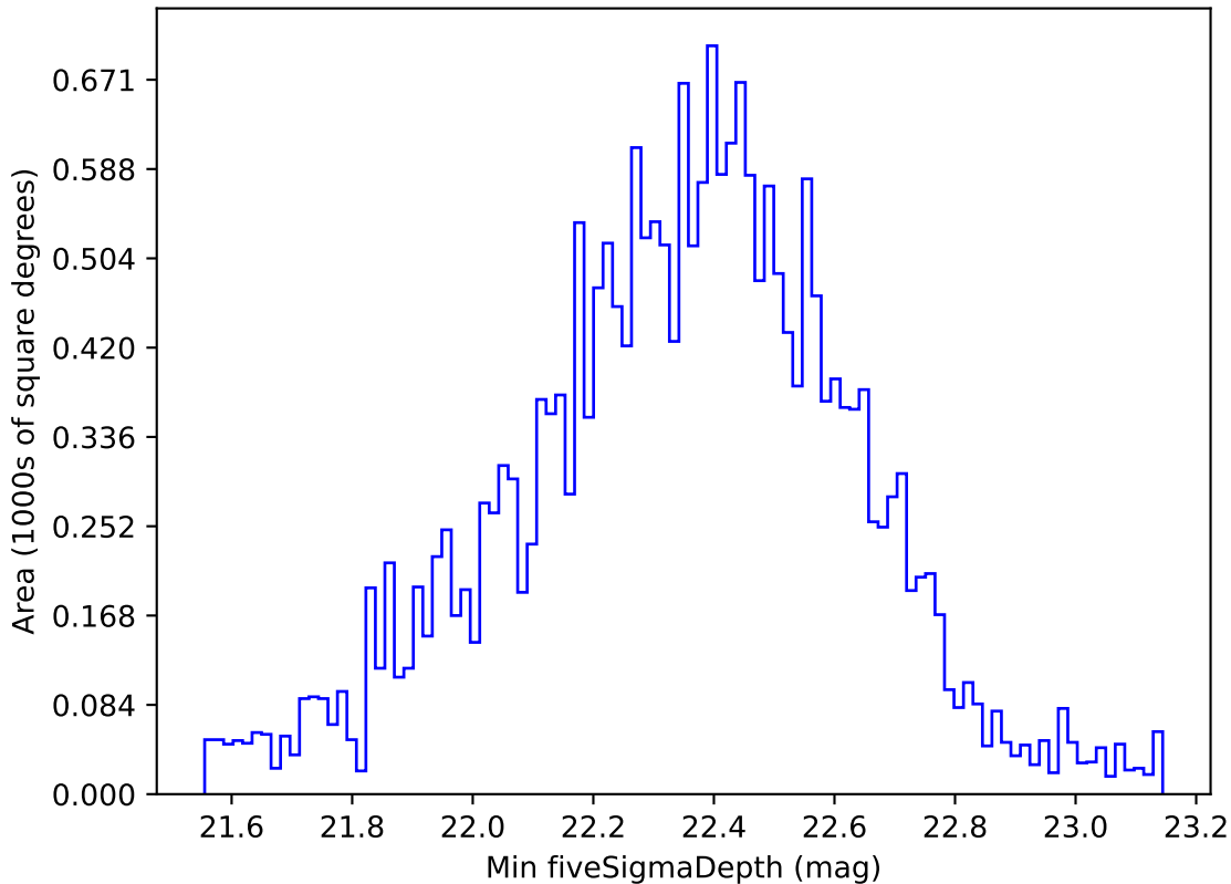
early_u_fpextra3.0_v3.4_10yrs All sky u band: Min fiveSigmaDepth
