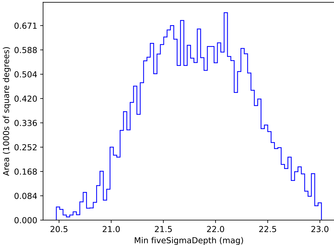
early_u_fpextra3.0_v3.4_10yrs All sky i band: Min fiveSigmaDepth
