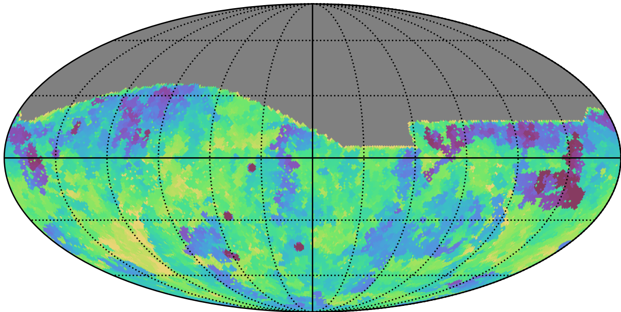
early_u_fpextra3.0_v3.4_10yrs All sky g band: Min fiveSigmaDepth
