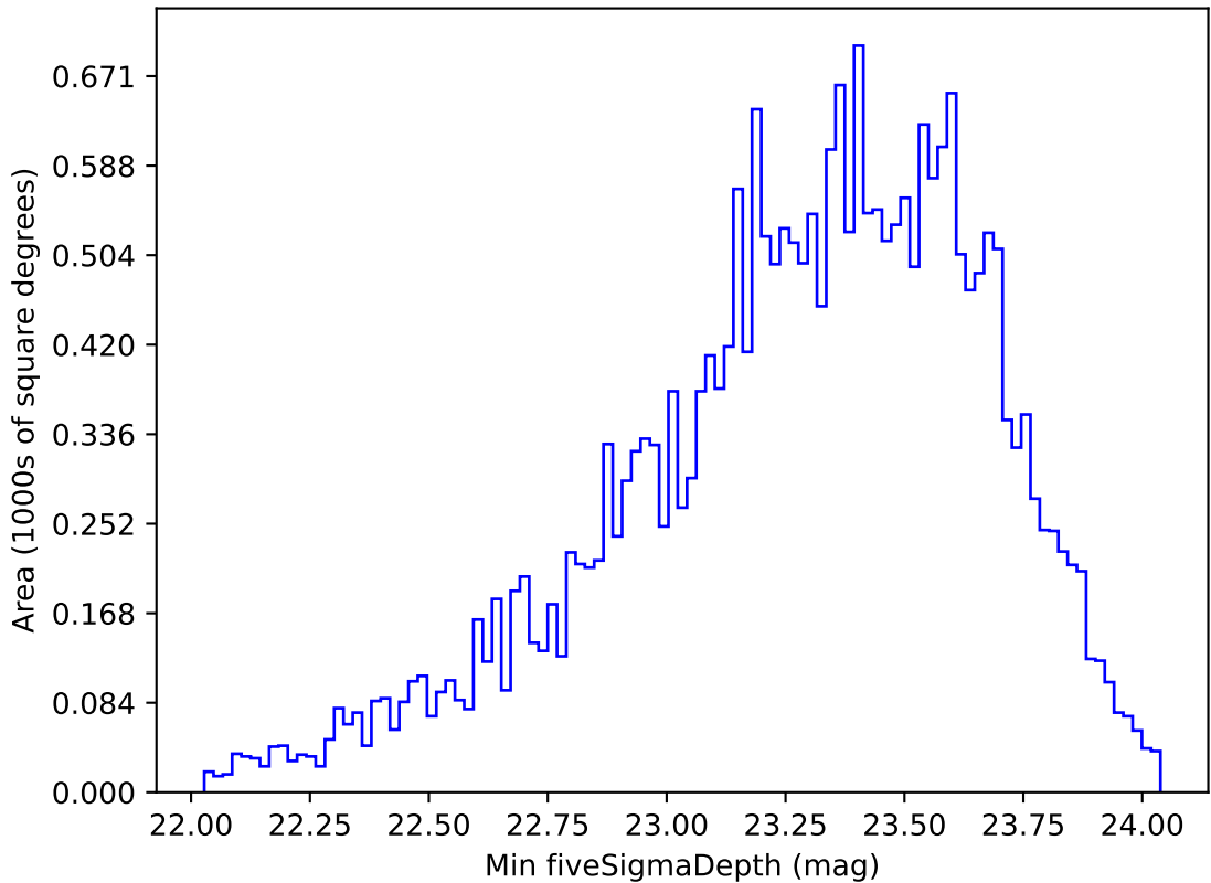
early_u_fpextra3.0_v3.4_10yrs All sky g band: Min fiveSigmaDepth
