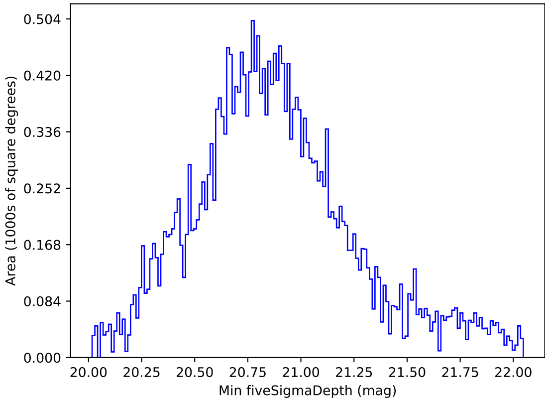
early_u_fpextra3.0_v3.4_10yrs All sky all bands: Min fiveSigmaDepth
