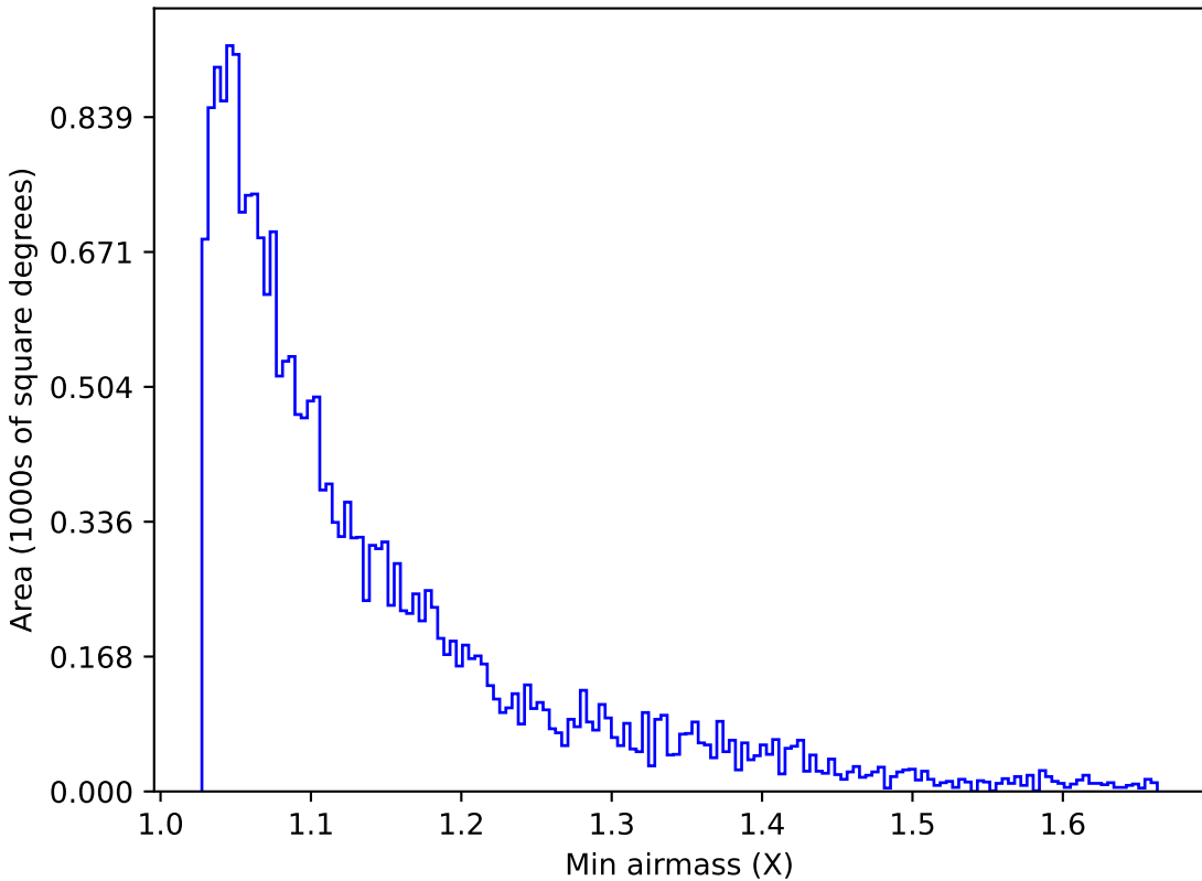
early_u_fpextra3.0_v3.4_10yrs Yr 1 u band: Min airmass
