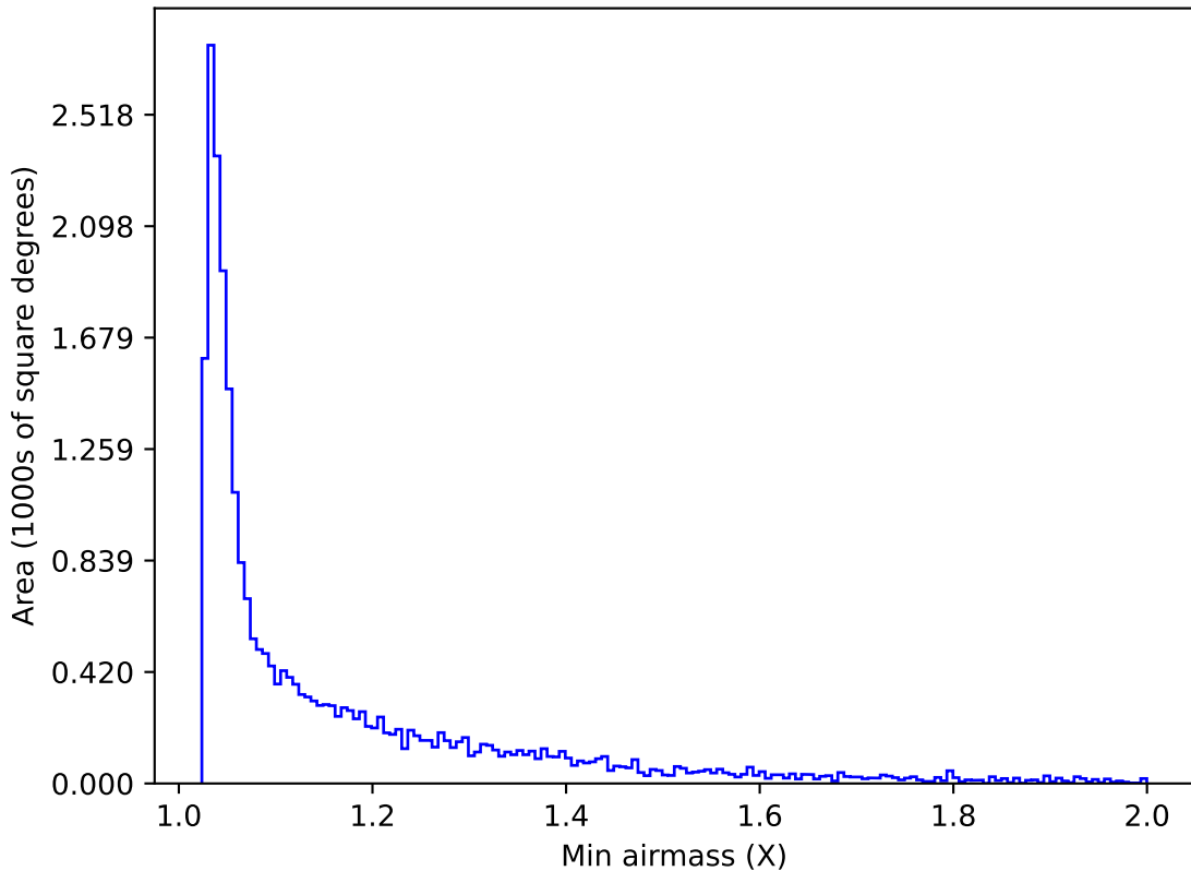
early_u_fpextra3.0_v3.4_10yrs Yr 1 r band: Min airmass
