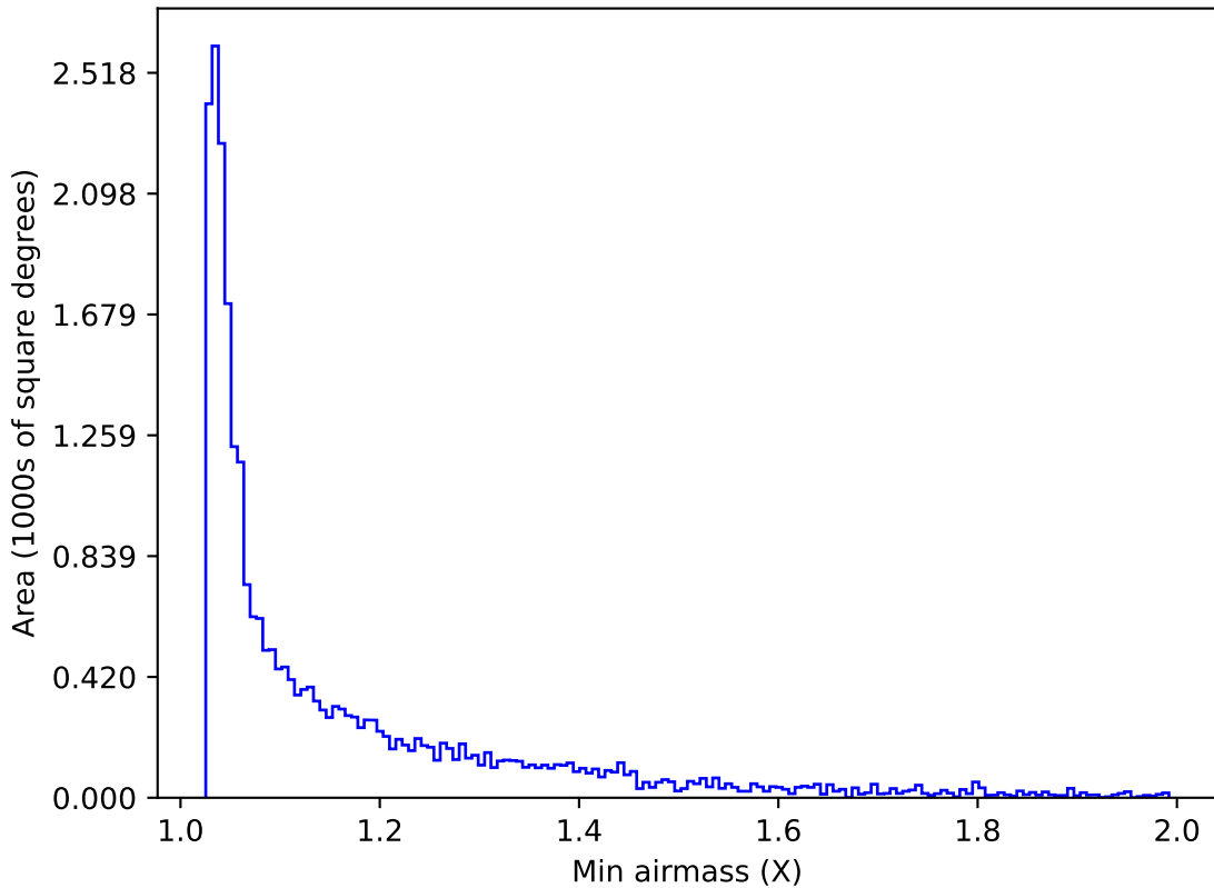
early_u_fpextra3.0_v3.4_10yrs Yr 1 i band: Min airmass
