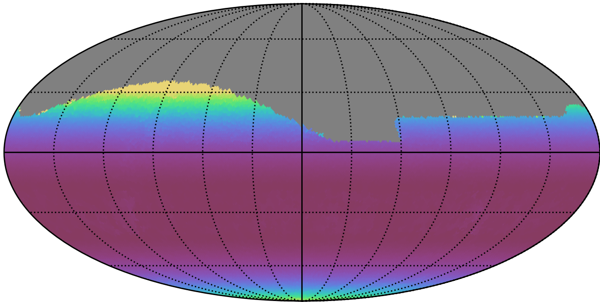
early_u_fpextra3.0_v3.4_10yrs Yr 1 all bands: Min airmass
