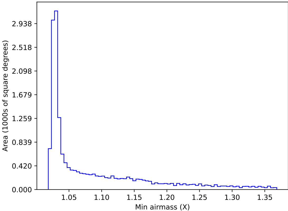
early_u_fpextra3.0_v3.4_10yrs WFD z band: Min airmass
