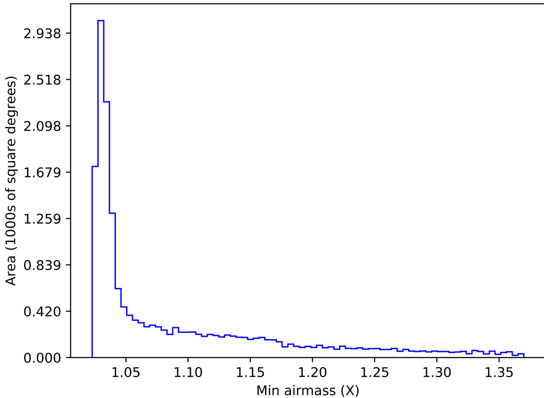
early_u_fpextra3.0_v3.4_10yrs WFD y band: Min airmass
