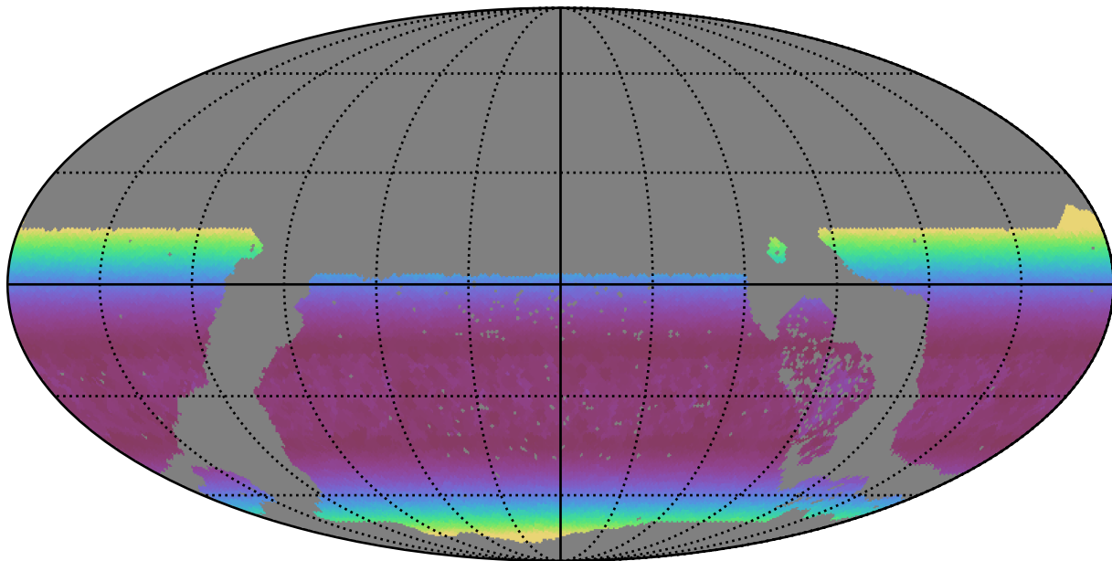
early_u_fpextra3.0_v3.4_10yrs WFD u band: Min airmass
