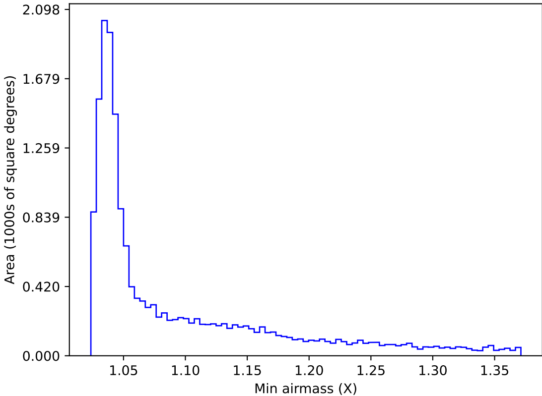
early_u_fpextra3.0_v3.4_10yrs WFD u band: Min airmass
