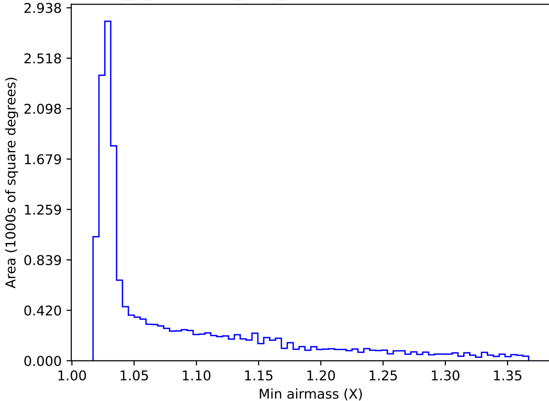
early_u_fpextra3.0_v3.4_10yrs WFD r band: Min airmass
