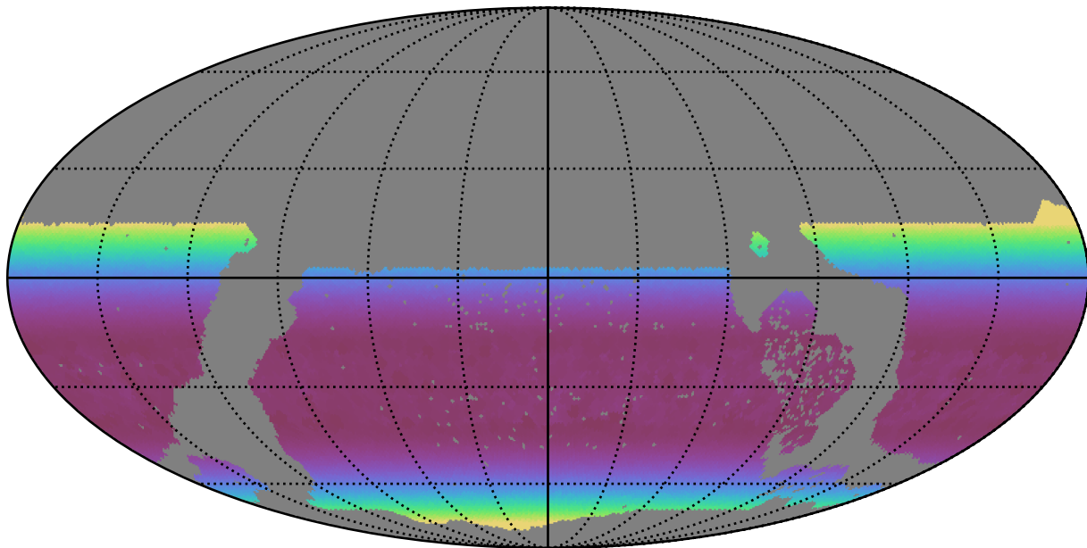
early_u_fpextra3.0_v3.4_10yrs WFD i band: Min airmass
