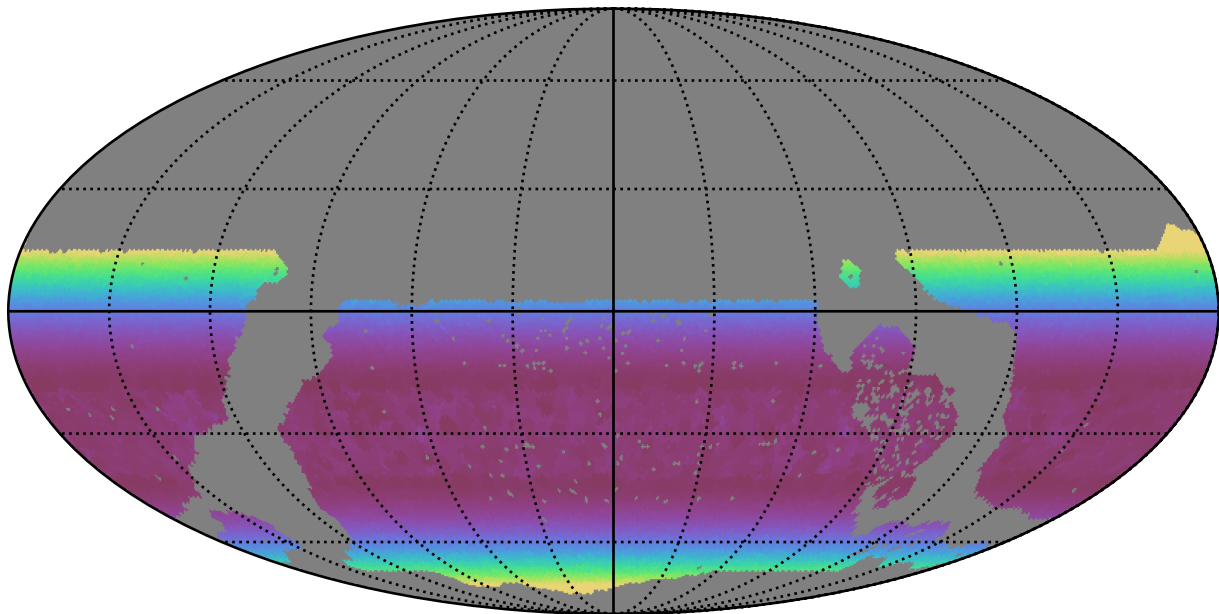
early_u_fpextra3.0_v3.4_10yrs WFD g band: Min airmass
