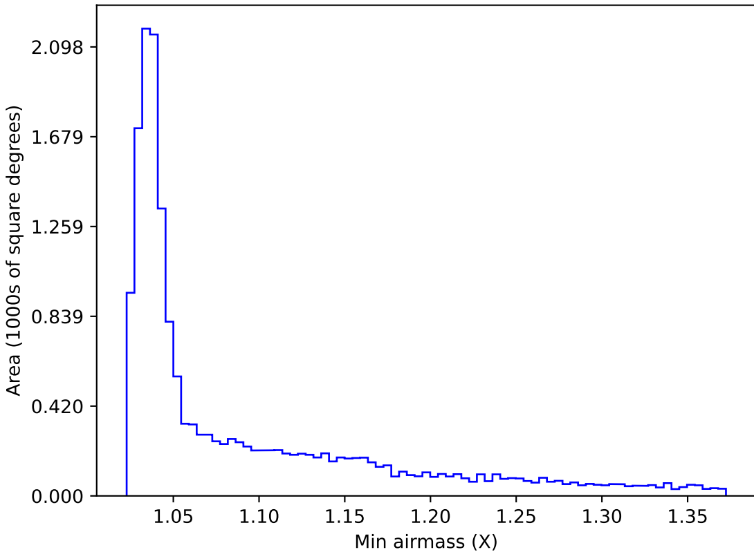
early_u_fpextra3.0_v3.4_10yrs WFD g band: Min airmass
