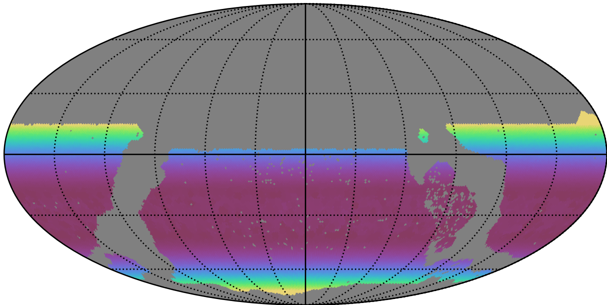
early_u_fpextra3.0_v3.4_10yrs WFD all bands: Min airmass
