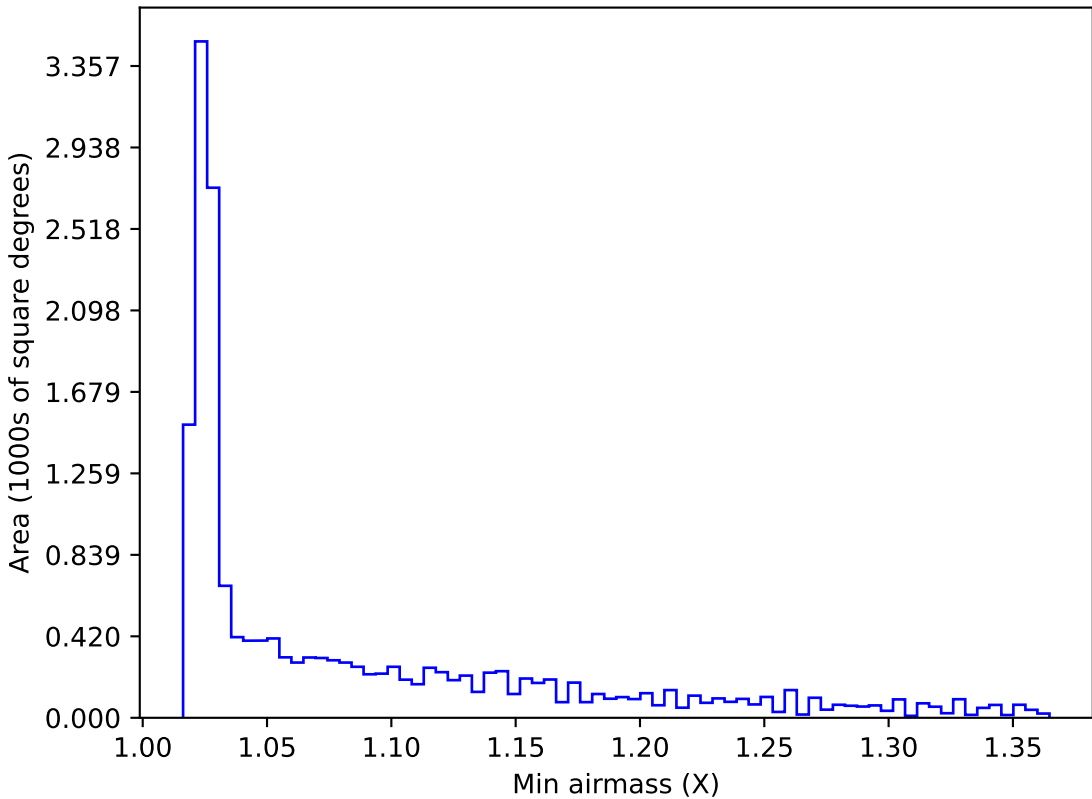
early_u_fpextra3.0_v3.4_10yrs WFD all bands: Min airmass
