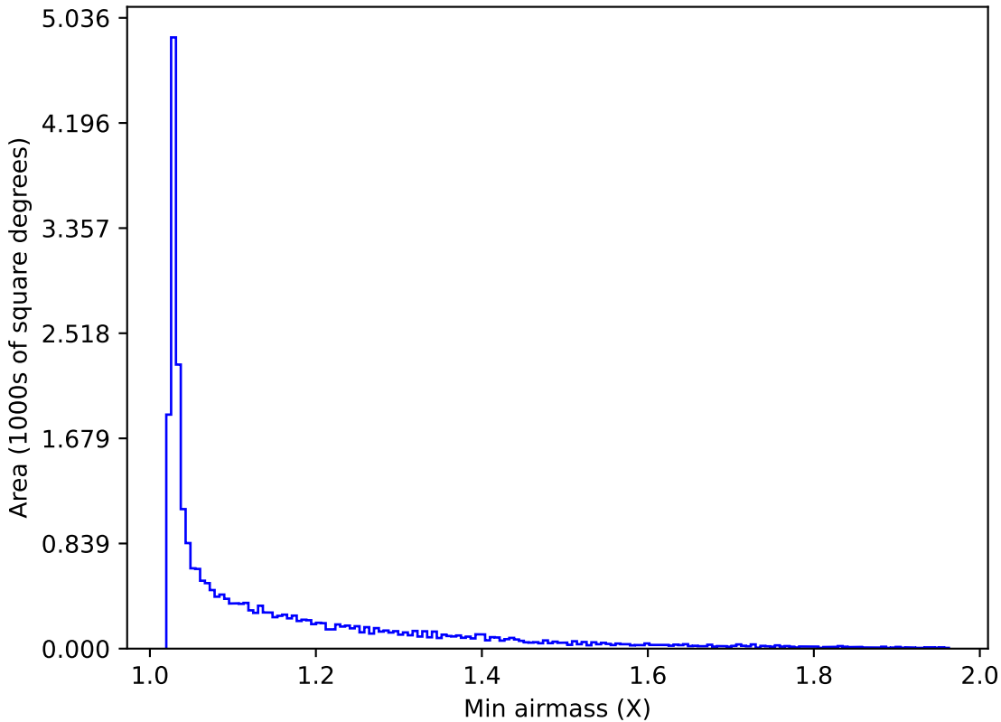
early_u_fpextra3.0_v3.4_10yrs All sky z band: Min airmass
