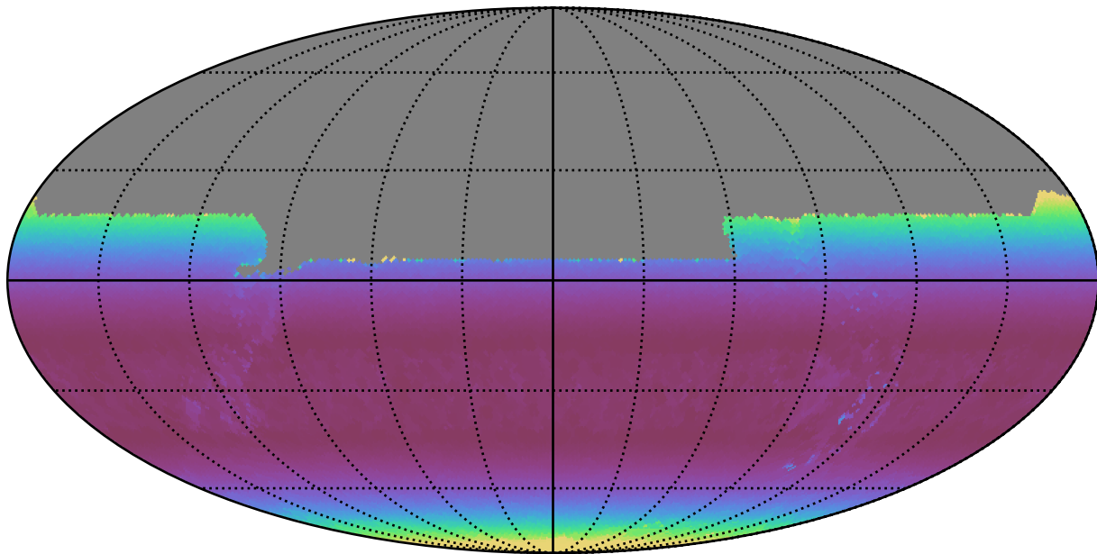
early_u_fpextra3.0_v3.4_10yrs All sky u band: Min airmass
