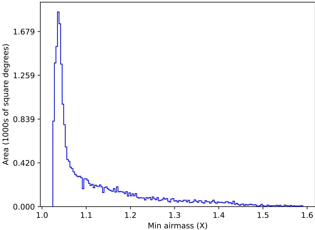
early_u_fpextra3.0_v3.4_10yrs All sky u band: Min airmass
