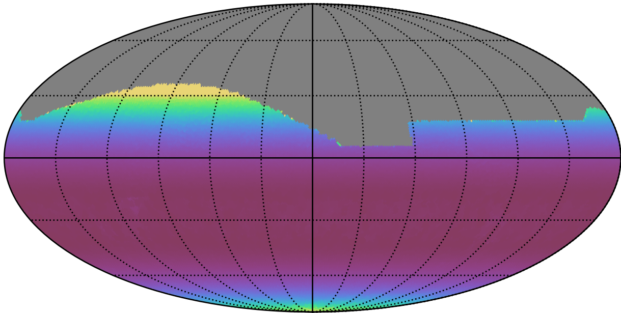
early_u_fpextra3.0_v3.4_10yrs All sky r band: Min airmass
