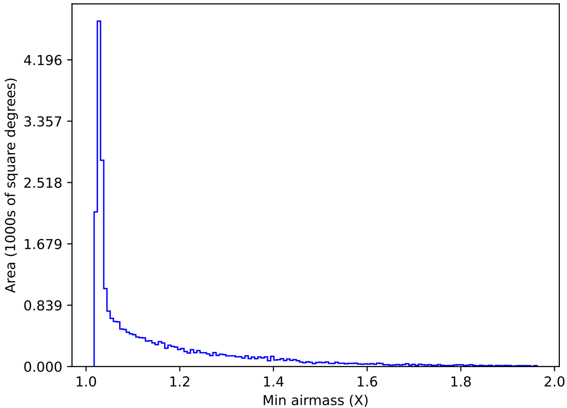
early_u_fpextra3.0_v3.4_10yrs All sky r band: Min airmass
