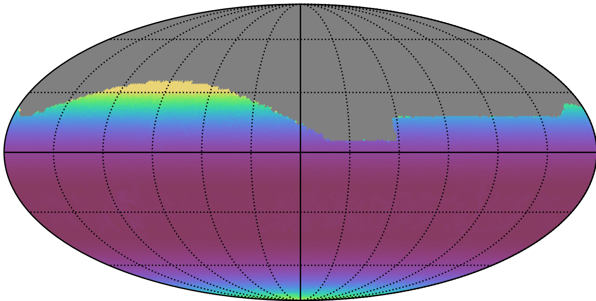
early_u_fpextra3.0_v3.4_10yrs All sky i band: Min airmass
