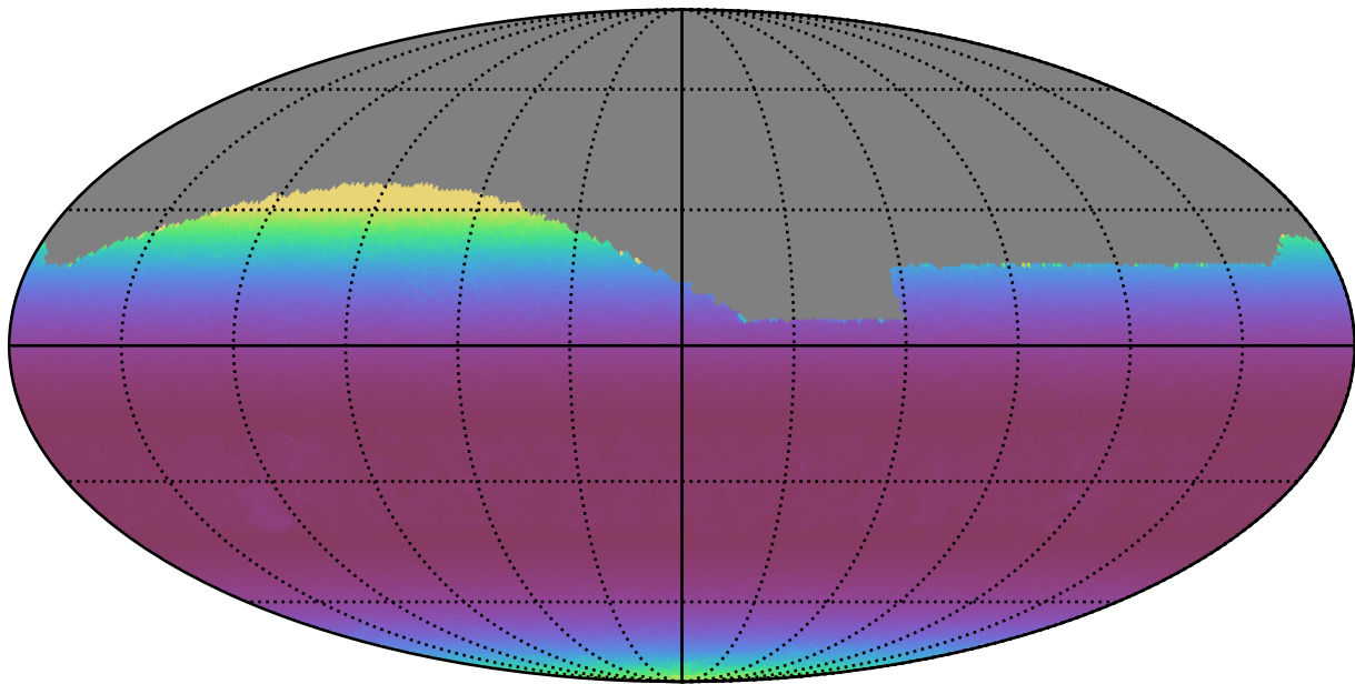
early_u_fpextra3.0_v3.4_10yrs All sky g band: Min airmass
