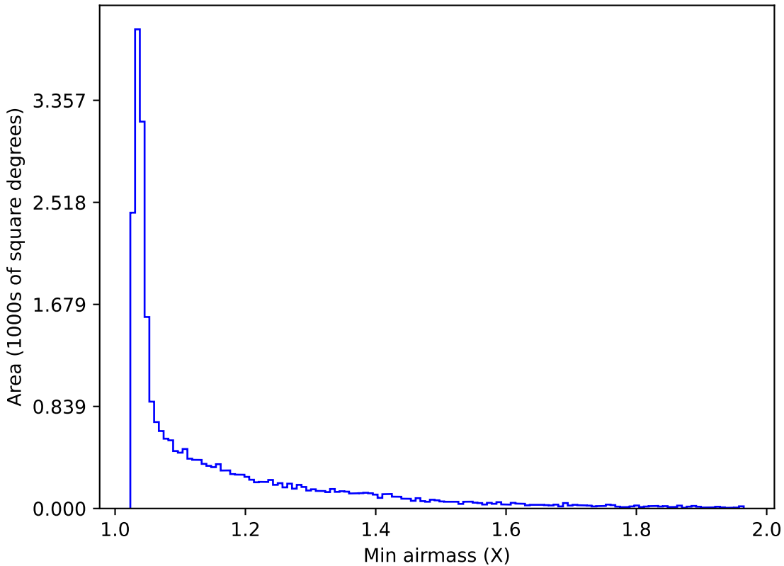
early_u_fpextra3.0_v3.4_10yrs All sky g band: Min airmass
