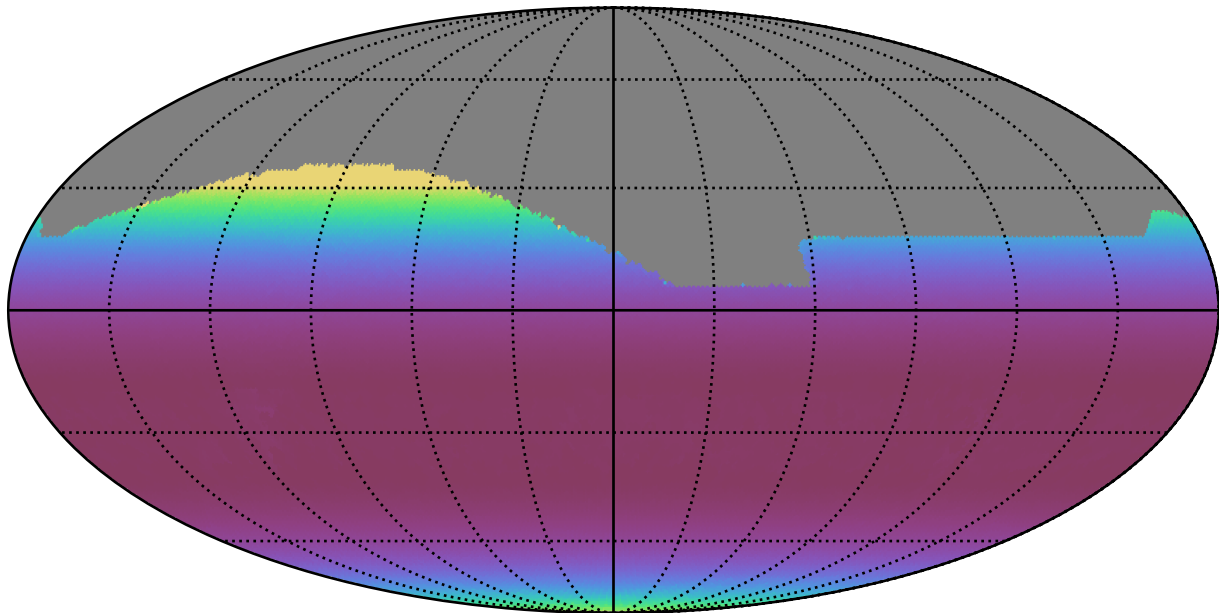
early_u_fpextra3.0_v3.4_10yrs All sky all bands: Min airmass
