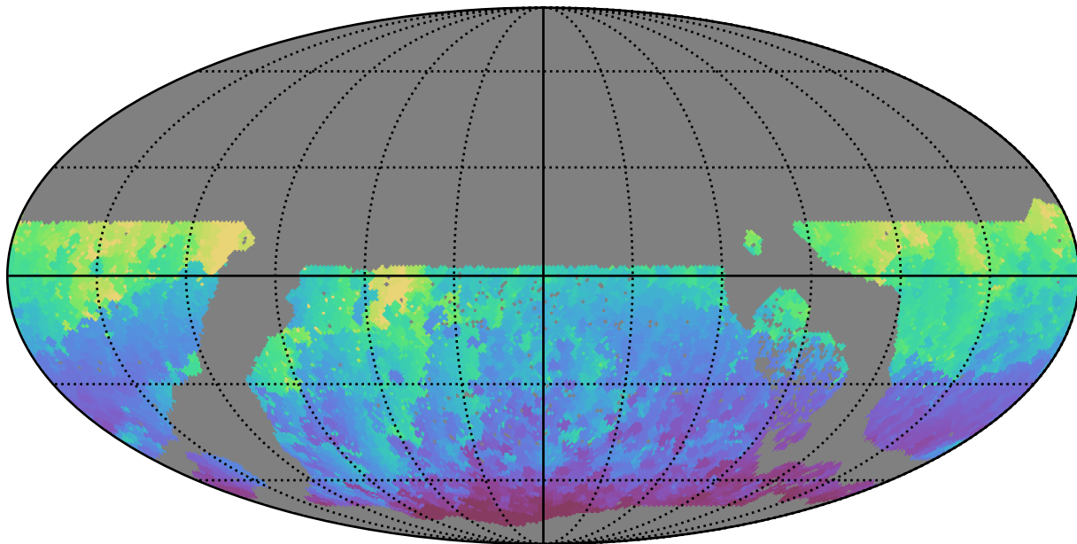
early_u_fpextra3.0_v3.4_10yrs WFD z band: Min HA
