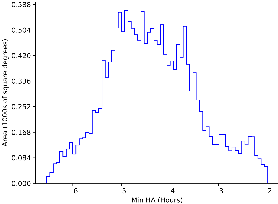
early_u_fpextra3.0_v3.4_10yrs WFD z band: Min HA
