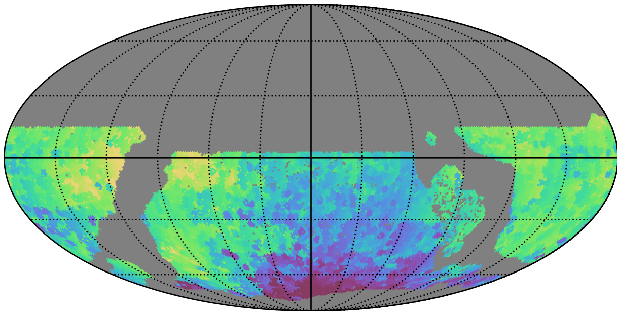
early_u_fpextra3.0_v3.4_10yrs WFD y band: Min HA
