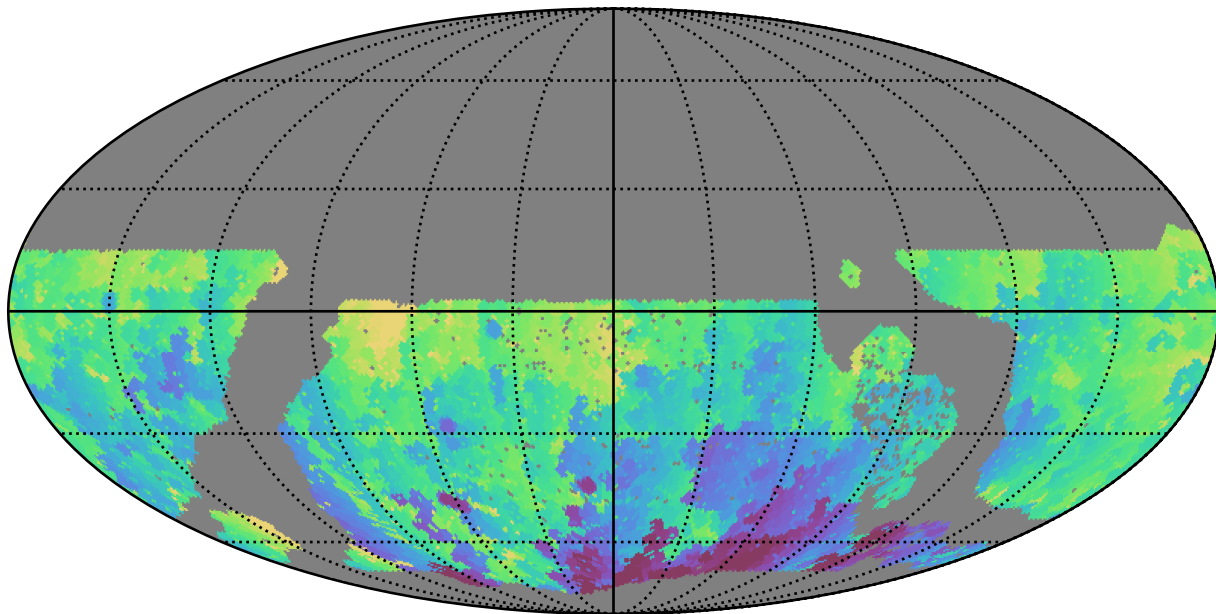
early_u_fpextra3.0_v3.4_10yrs WFD u band: Min HA
