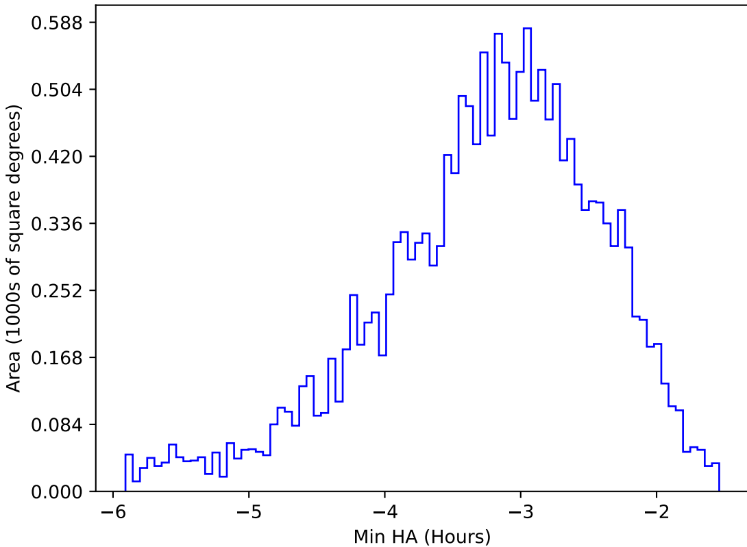
early_u_fpextra3.0_v3.4_10yrs WFD u band: Min HA
