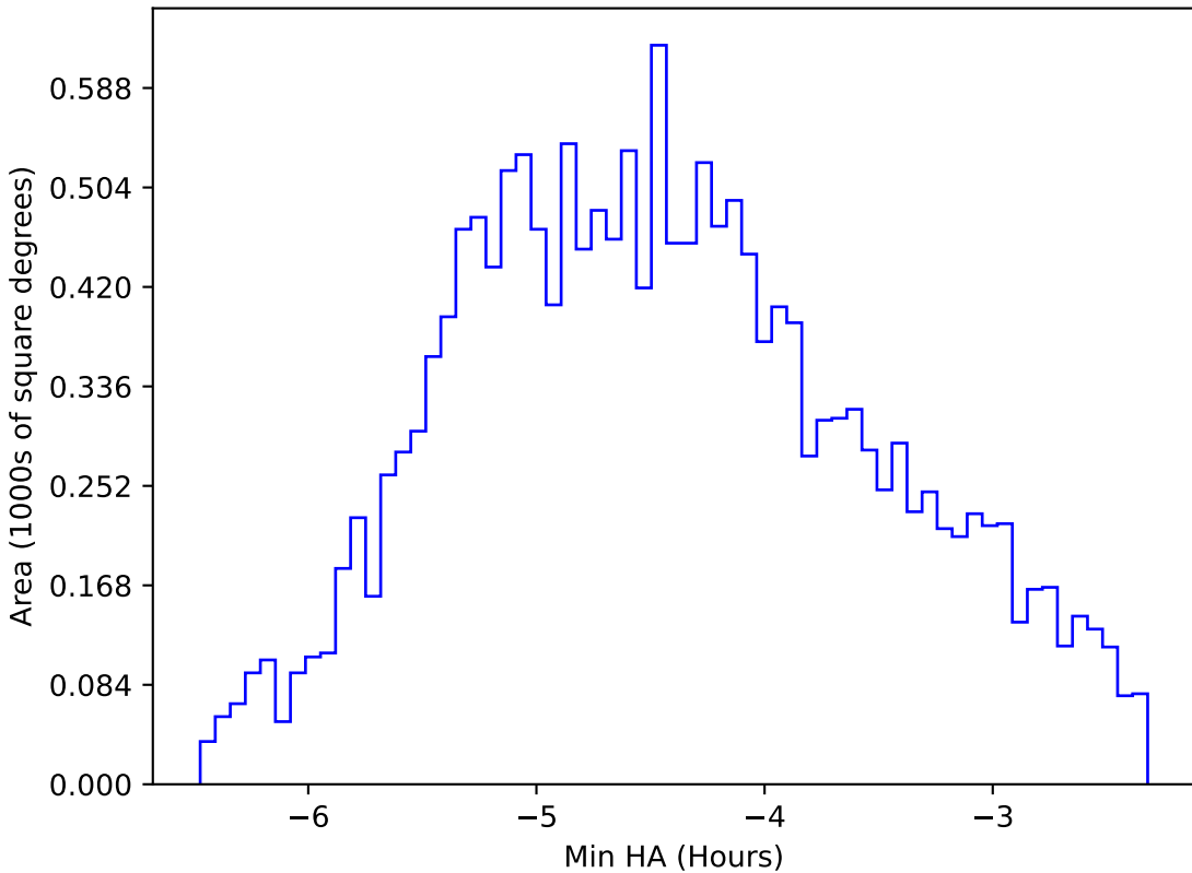
early_u_fpextra3.0_v3.4_10yrs WFD r band: Min HA
