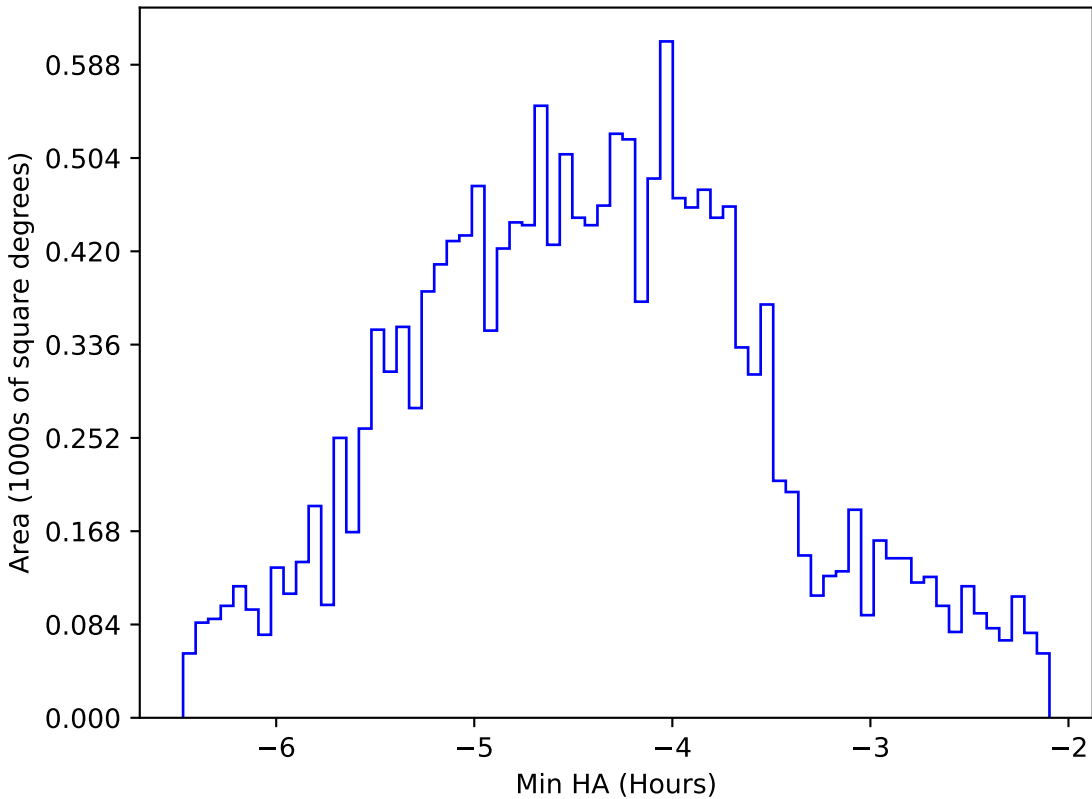
early_u_fpextra3.0_v3.4_10yrs WFD i band: Min HA
