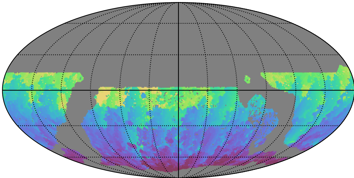
early_u_fpextra3.0_v3.4_10yrs WFD g band: Min HA
