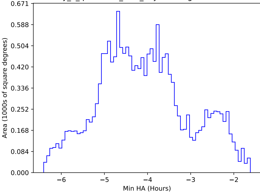
early_u_fpextra3.0_v3.4_10yrs WFD g band: Min HA
