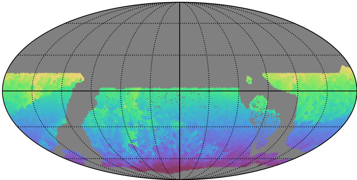
early_u_fpextra3.0_v3.4_10yrs WFD all bands: Min HA
