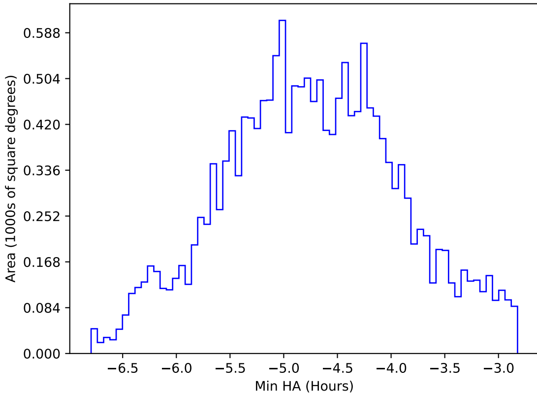
early_u_fpextra3.0_v3.4_10yrs WFD all bands: Min HA
