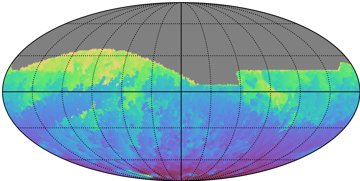
early_u_fpextra3.0_v3.4_10yrs All sky z band: Min HA
