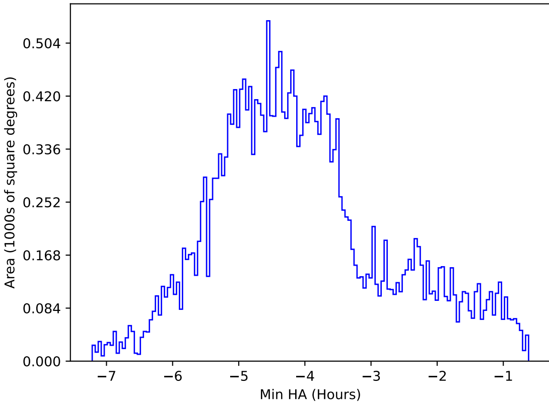
early_u_fpextra3.0_v3.4_10yrs All sky z band: Min HA
