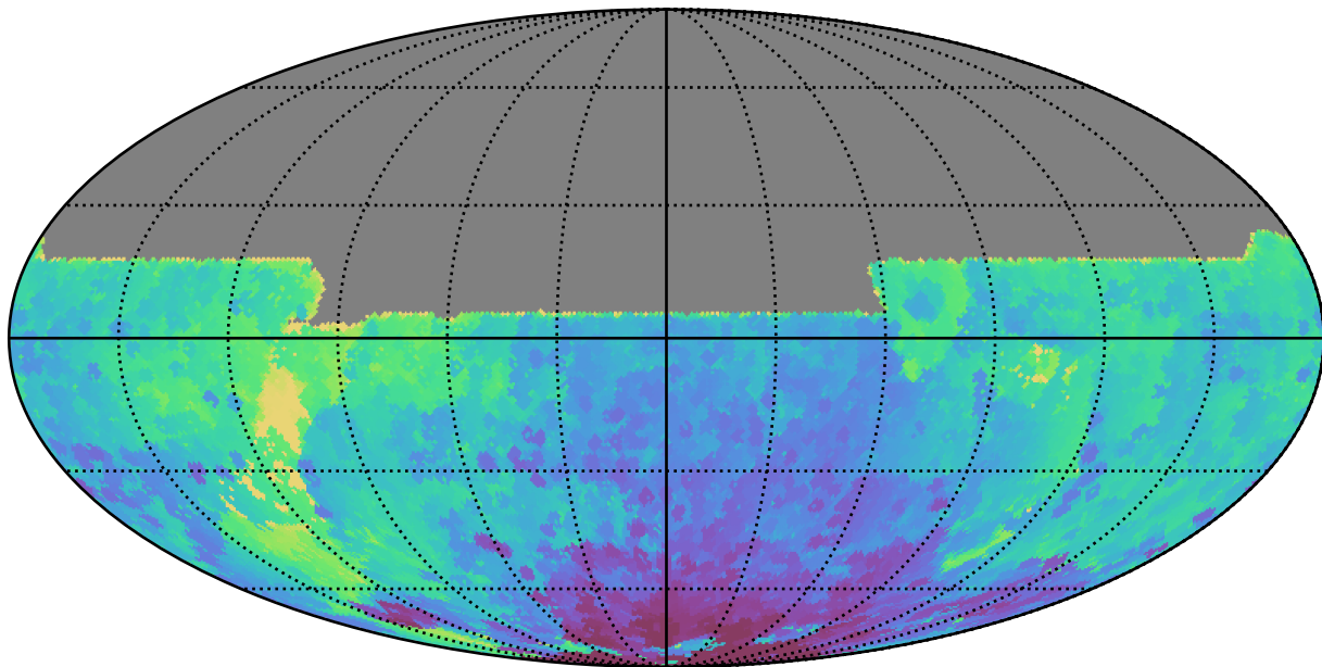
early_u_fpextra3.0_v3.4_10yrs All sky y band: Min HA
