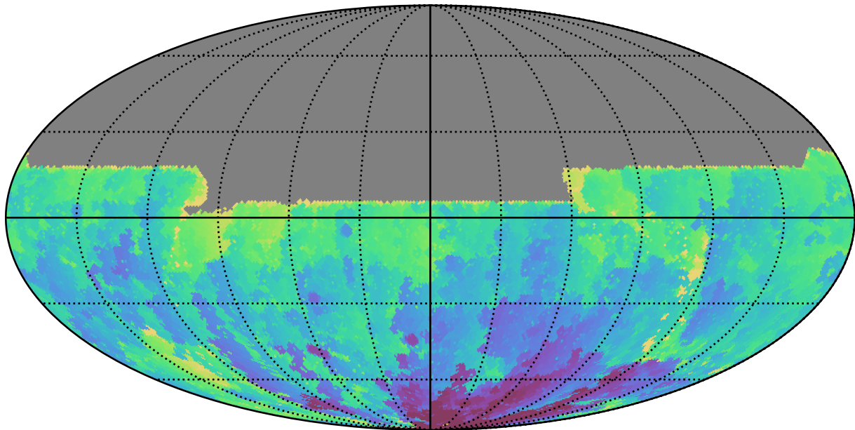
early_u_fpextra3.0_v3.4_10yrs All sky u band: Min HA
