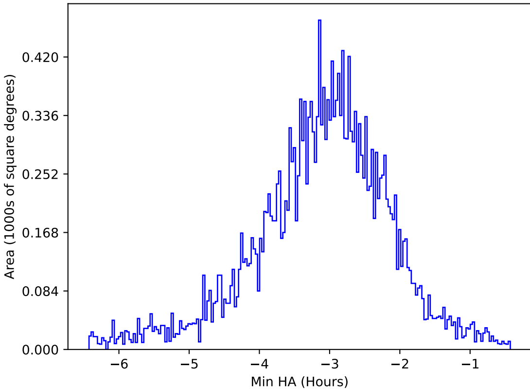
early_u_fpextra3.0_v3.4_10yrs All sky u band: Min HA
