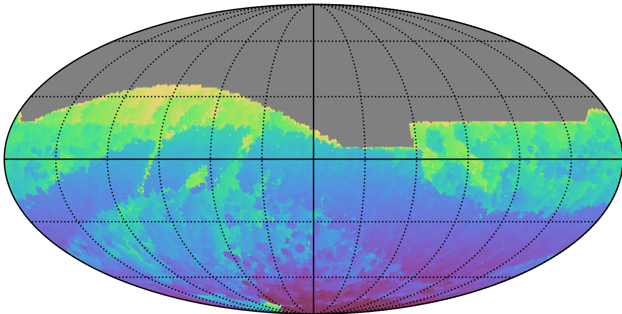
early_u_fpextra3.0_v3.4_10yrs All sky r band: Min HA
