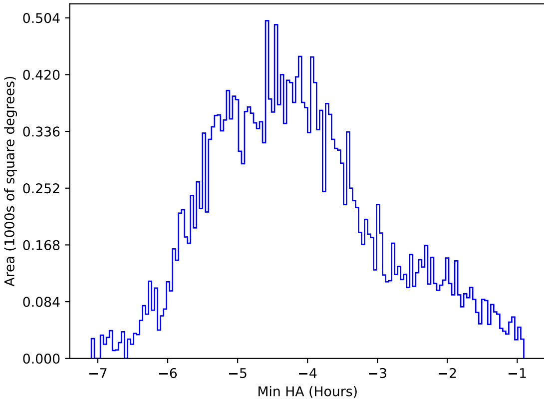
early_u_fpextra3.0_v3.4_10yrs All sky r band: Min HA
